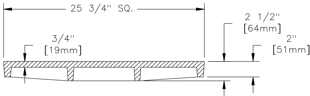
COVER SECTION
