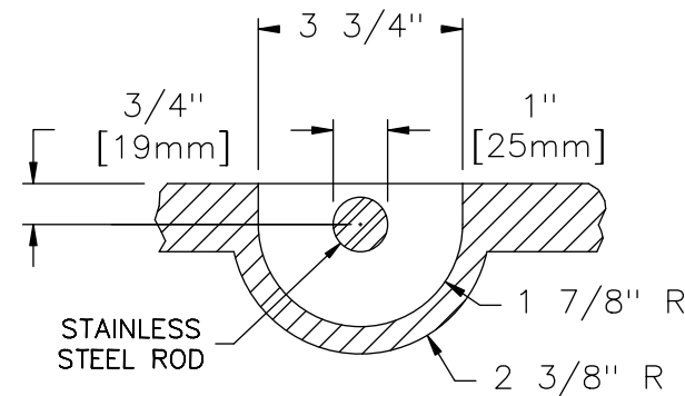
PICKBAR DETAIL
